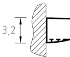
Wall profiles dimensions
